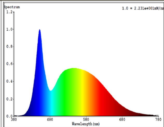
EBE-BAQ501-9W E27 (6500K): 1#
